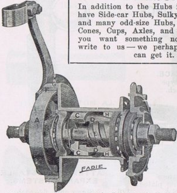
6/11—Showing Internal Parts of Eadie Coaster Hub.
