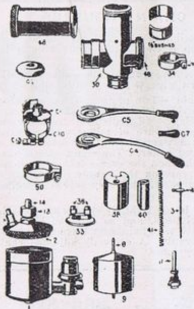
63/17—CARBURETTOR PARTS.
