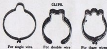
27/13—BOWDEN FRAME CLIPS.
