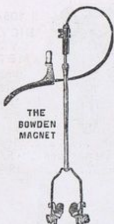
THE BOWDEN MAGNET 24/11. BOWDEN MAGNET BRAKES. Suits any shape bar. Front, 7/6 ea. complete Rear, 10/- ea. complete
