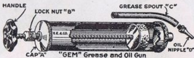
45/10—"GEM" COMBINATION GREASE AND OIL GUN.
