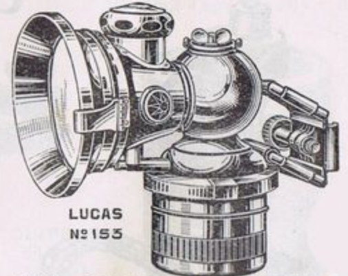
75/28— LUCAS CALCIA TOURA. A medium-priced Lucas Lamp, embodying all modern improvements. Has a large front with an aluminium reflector and patented fixing for carbide container. The water body is fitted with combination water-filler, cap and funnel, which is not detachable. Complete with valve nipple for rear light. 25/- each.
