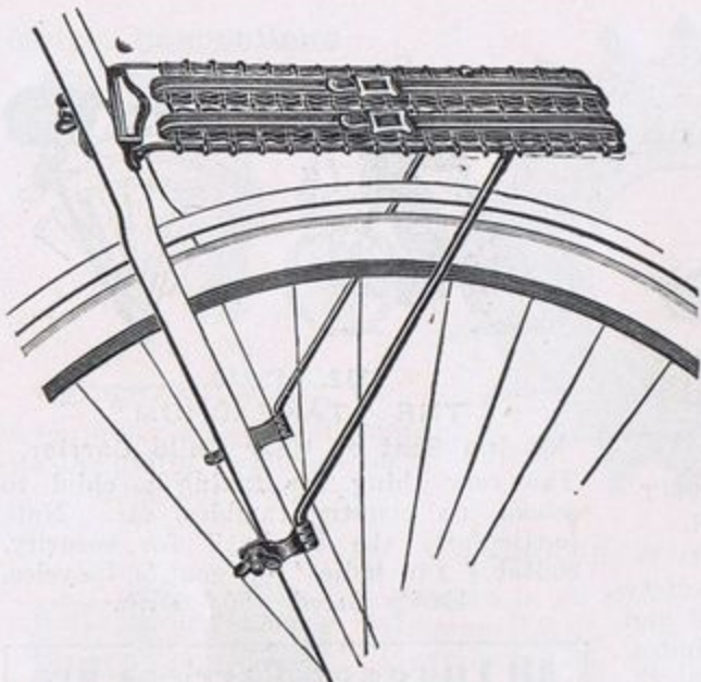
3/10. BLUEMEL'S CLIP-ON CARRIER.
