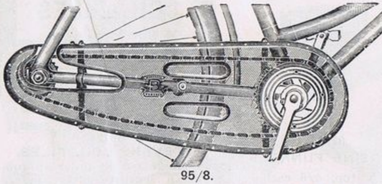
95/8. BLUEMEL FEATHERWEIGHT DETACHABLE CHAIN COVER.
