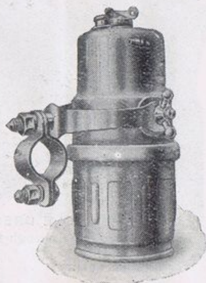
80/12. P. and H. DE LUXE MOTOR CYCLE GENERATOR. Large type, capable of carrying 9 \frac{1}{2} oz. carbide. Has a double carbide container with a simple but positive locking device for ensuring an absolute gas-tight joint. Fitted with adjustable carrier and two-way gas tap. Height 8", diameter 3 \frac{1}{2} "", weight 2lb. 6oz. Ebony with plated mounts. 25/- each.
