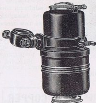
77/28. P. AND H. MOTOR CYCLE GENERATOR. This model has a swivel bail for holding carbide chamber in position and a positive gas-tight locking device. It has a carbide capacity of 10oz. and will supply a light for 5 hours. Fitted with two-way gas tap. Height 8 \frac{1}{2} "", diameter 3 \frac{3}{8} "", weight 2lb. 3oz. Ebony with plated mounts. 20/- each.
