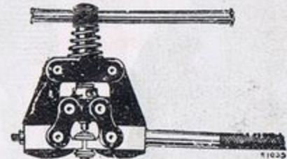
99/18— THE COVENTRY UNIVERSAL RIVET EXTRACTOR.
