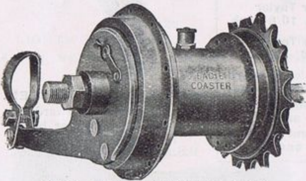
11/11—EADIE COASTER HUB.
