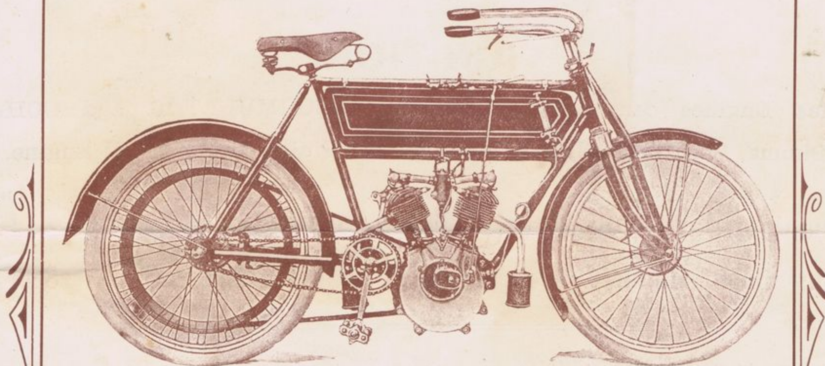
Illustrating 5 H.P. "SAROLEA," Two Cylinders.
