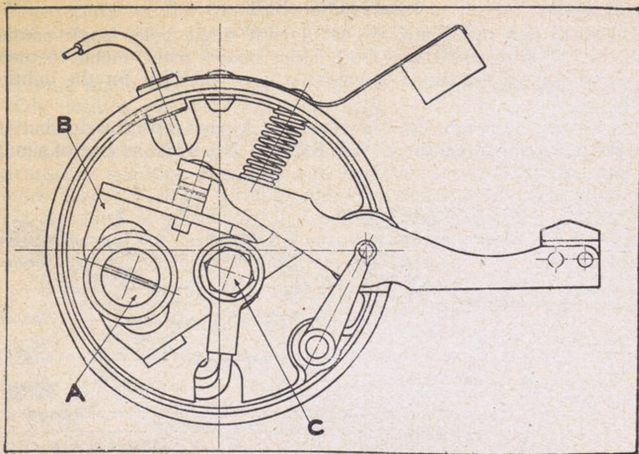
FIG. 2. CONTACT BREAKER ASSEMBLY.
