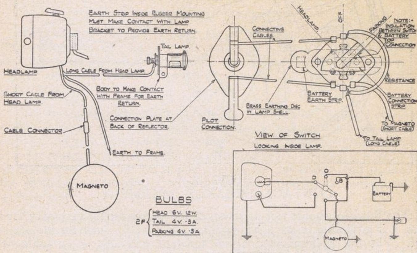
FIG. 3. WIRING DIAGRAM Mk. 2.F. TRACING TROUBLES.
